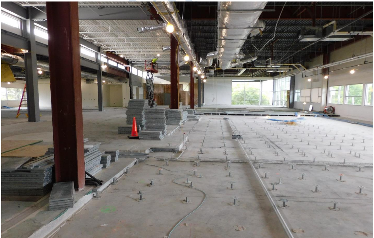
Data run pathway to new IDF/MDF room second floor serving as the hub for all communications
